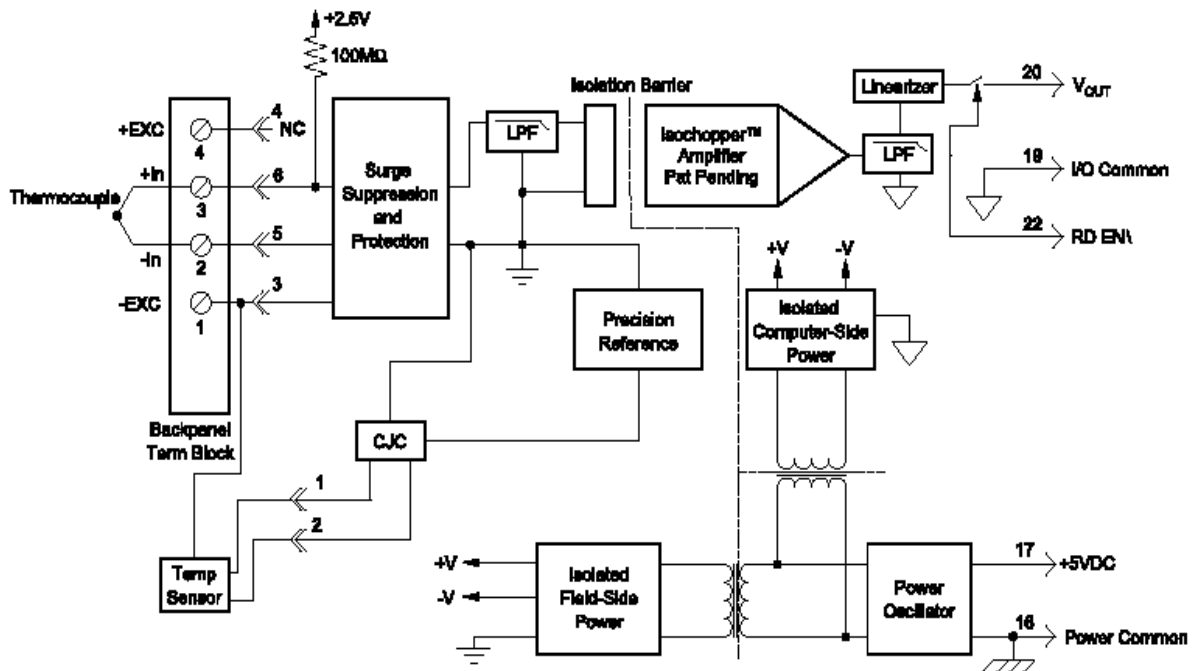
Figure 5 Dataforth's SCM5B47 Isolated Linearized Thermocouple Module
